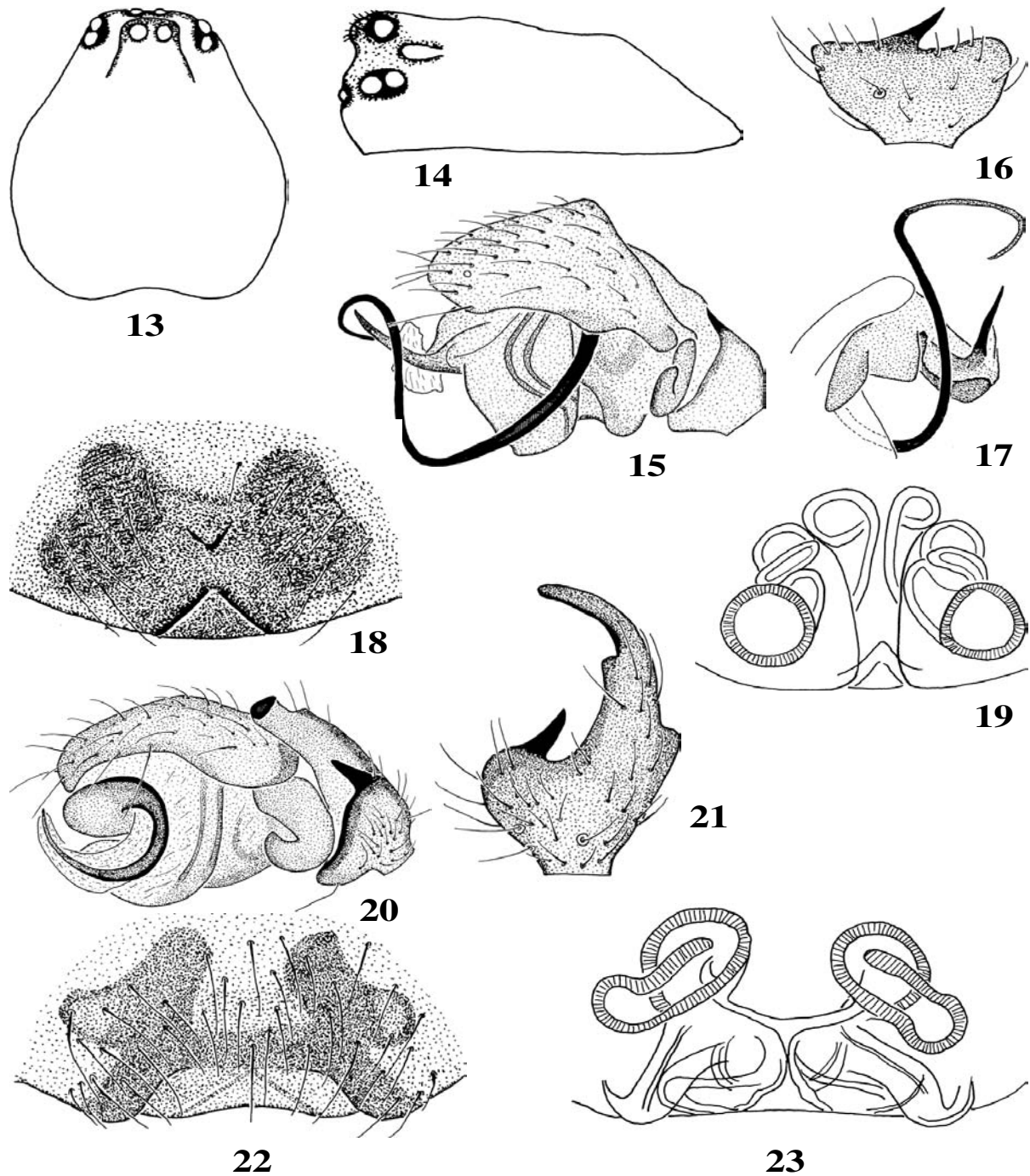
Figs 13-19. Silometopus nitidithorax Simon. Fig. 13. Male prosoma, dorsal view; 14. Idem, lateral view; 15. Male palp, retrolateral view; Fig. 16. Male palpal tibia, dorsal view; Fig. 17. Embolic division, prolateral view; Fig. 18. Epigyne, ventral view; Fig. 19. Vulva, ventral view. Figs 20-23. Walckenaeria abantensis Wunderlich. 20. Male palp, retrolateral view; 21. Male palpal tibia, dorsal view; 22. Epigyne, ventral view; 23. Vulva, ventral view.
