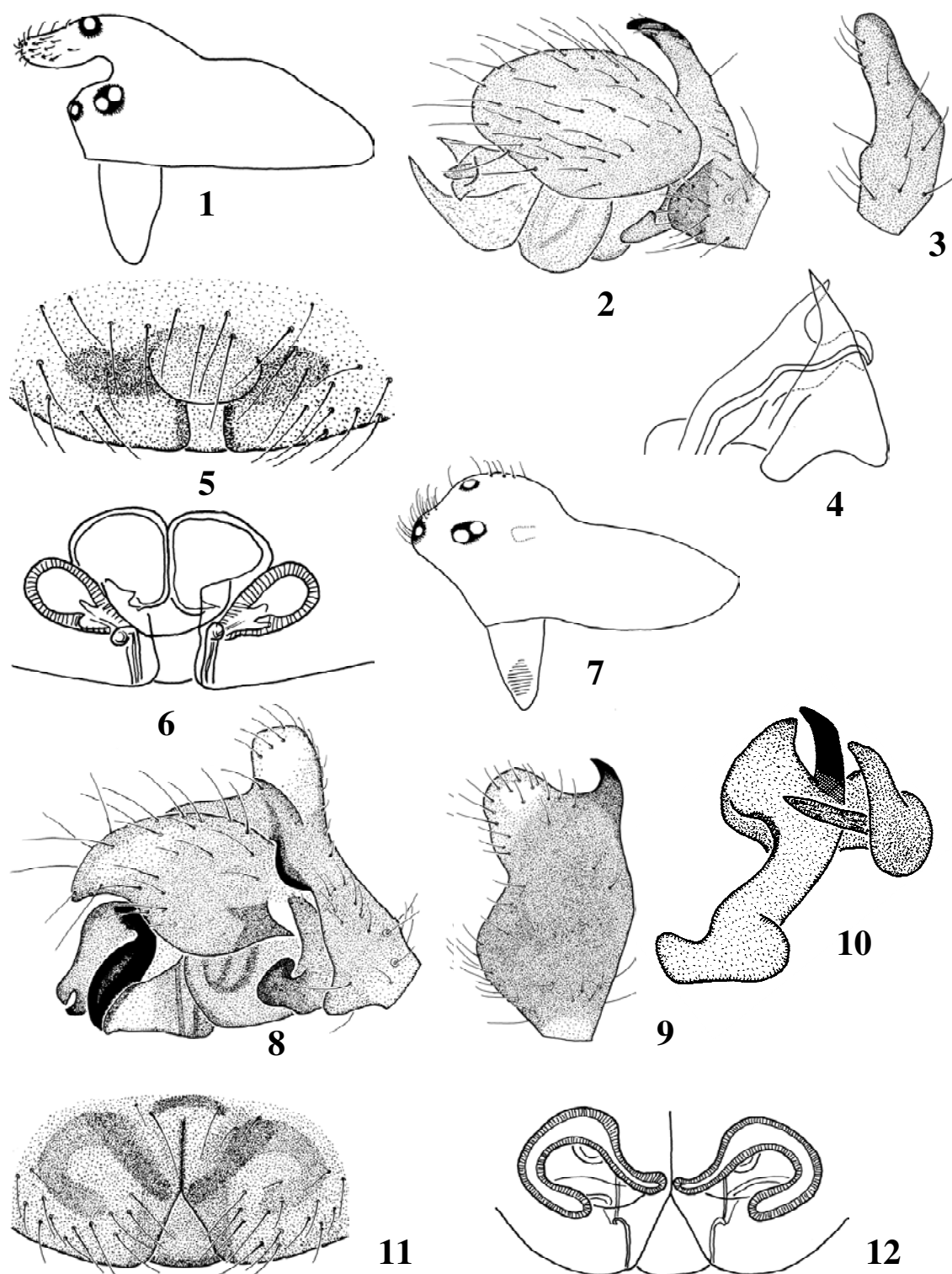
Figs 1-6. Dactylopisthes digiticeps (Simon). 1. Male prosoma, lateral view; 2. Male palp, retrolateral view; 3. Male palpal tibia, dorsal view; 4. Embolic division and suprategular apophysis, prolateral view; 5. Epigyne, ventral view; 6. Vulva, ventral view.
